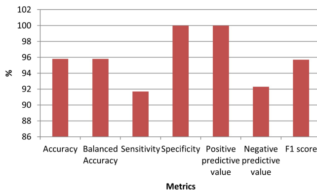
Figure 3. Graph for performance metrics obtained from XGboost models.
