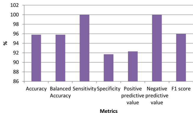
Figure 1. Graph for performance metrics obtained from XGboost models.
